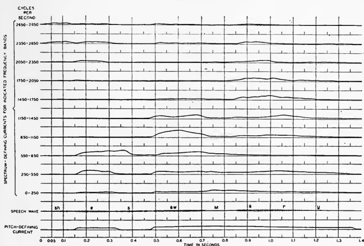
FIG. 3. The original speech wave and an analysis of its components, expressed by the variation of several direct currents.
